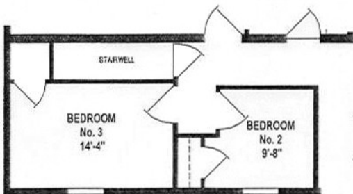
OPTION MODULAR STAIRWELL
